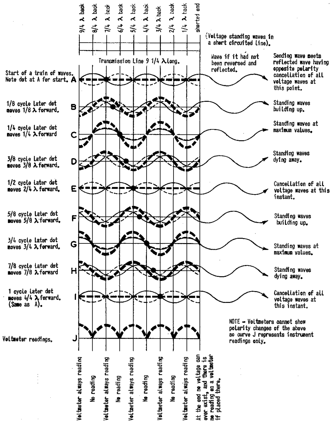
Fig. 3 - Process of building up standing waves of voltage in a transmission line terminated in a short circuit.
