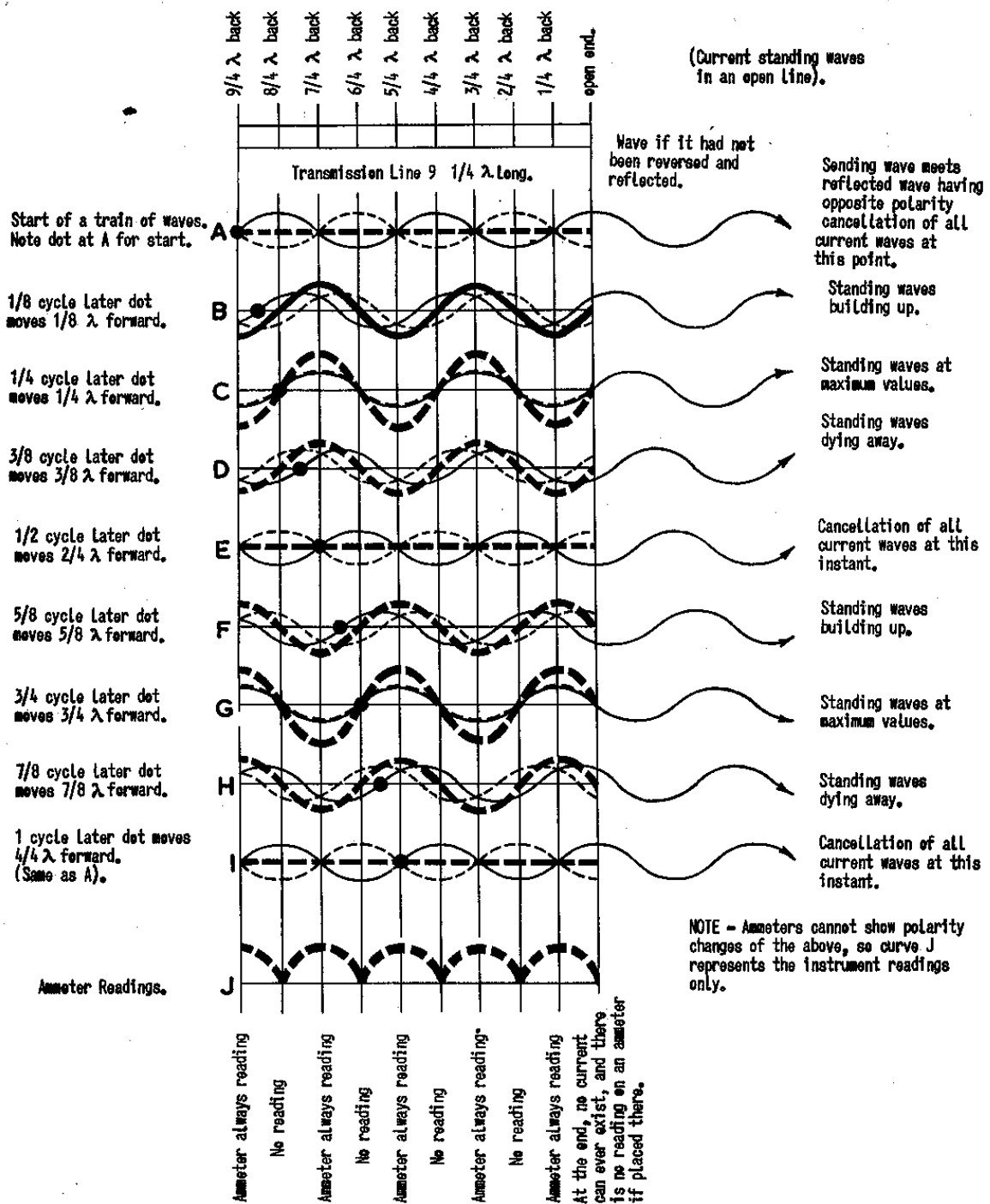
Fig. 2 - Process of building up standing waves of current in a transmission line terminated in an open circuit.
