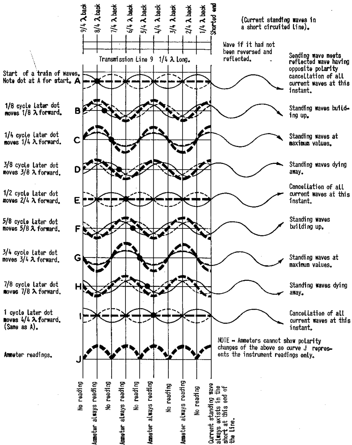
Fig. 4 - Process of building up standing waves of current in a transmission line terminated in a short circuit.
