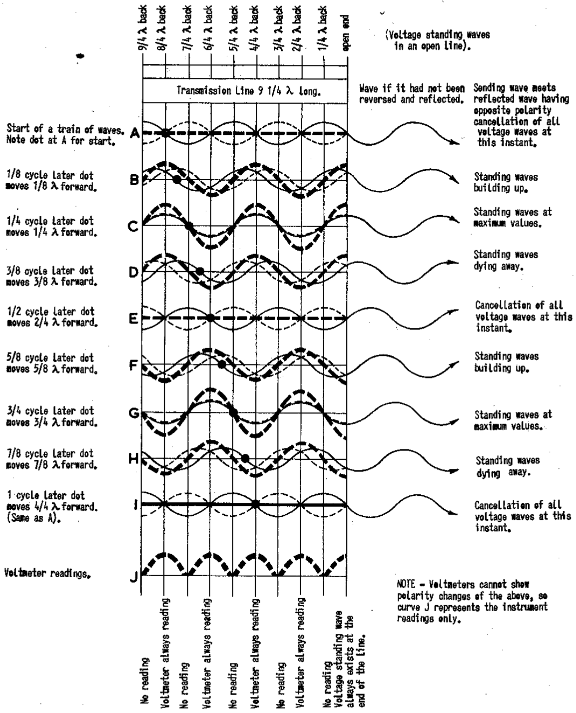
Fig. 1 - Process of building up standing waves of voltage in a transmission line terminated in an open circuit.
