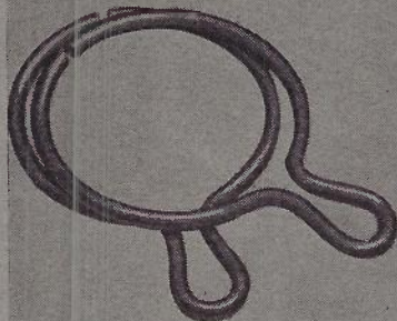
Picture Shift Magnets in 6% Chromium Steel
