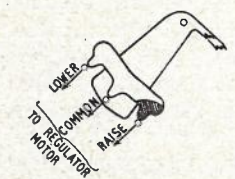
FIG. 2.—NO-VOLT PROTECTION.
