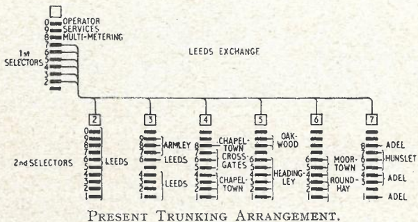
PRESENT TRUNKING ARRANGEMENT.
