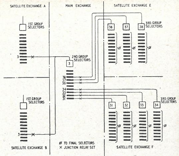
FIG. 4.—TRUNKING FOR SATELLITE EXCHANGES WITH THE SAME INITIAL DIGIT; SCHEME WITH ROUTING VIA MAIN EXCHANGE.
