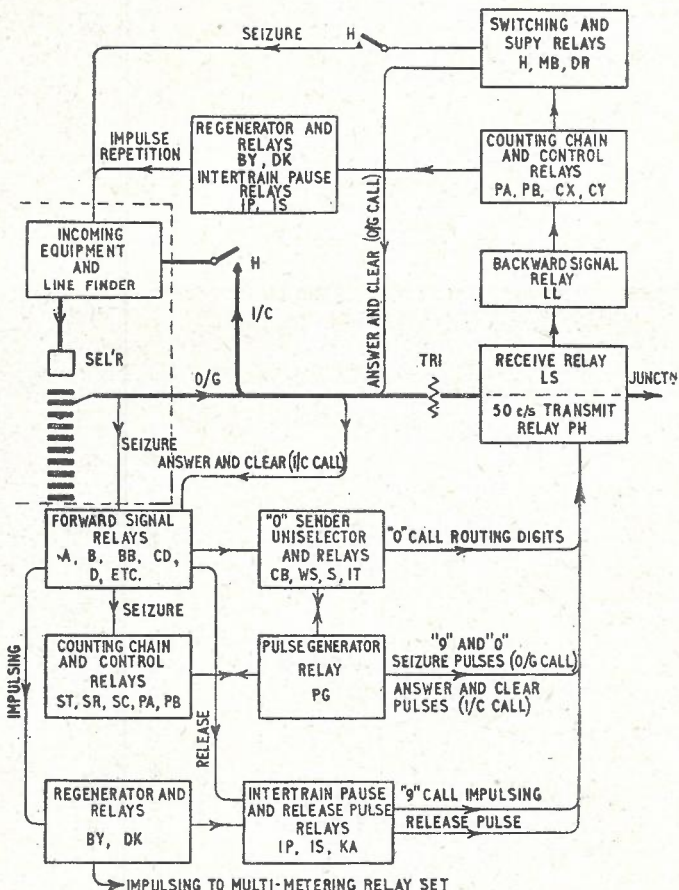
FIG. 2.—BLOCK SCHEMATIC DIAGRAM OF AUTO-AUTO RELAY SET.
