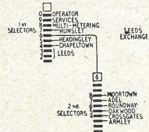
PROPOSED TRUNKING ARRANGEMENT.
