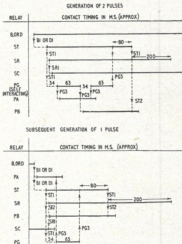
FIG. 5.—RELAY SEQUENCE OF FORWARD PULSE GENERATION.
