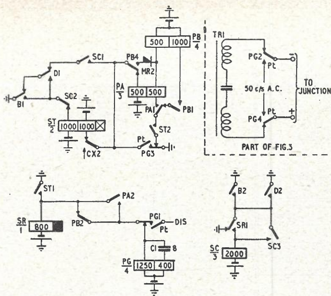
FIG. 4.—FORWARD PULSE SIGNALLING CIRCUIT ELEMENTS.
