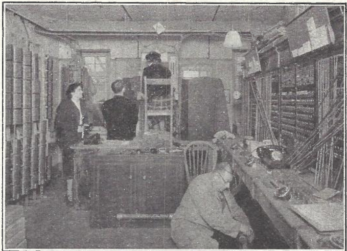
P.B.X. 10 + 50 MOUNTED ON PLATFORM IN CANVEY EXCHANGE.
