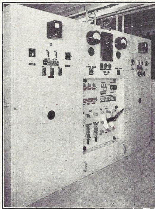
FIG. 5.—A 200-AMP. POWER PLANT, FRONT VIEW.
