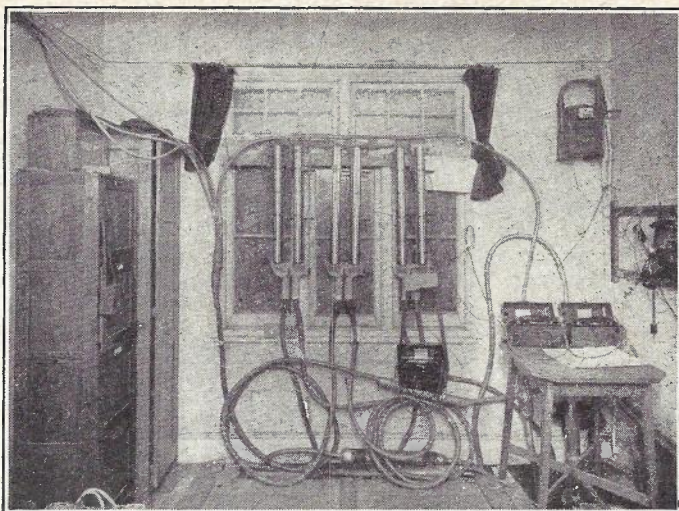
TEMPORARY CABLE TERMINATIONS AT CANVEY EXCHANGE.
